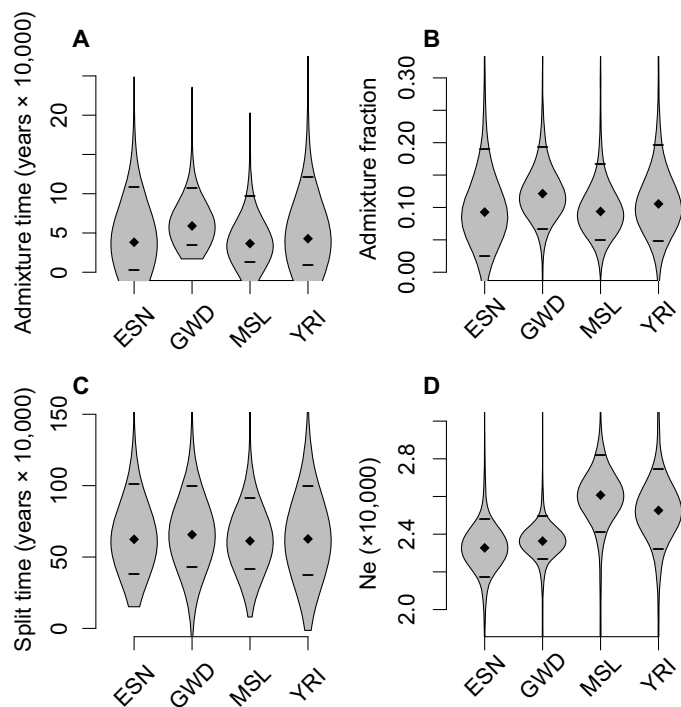
Fig. 2. ABC estimates of the demographic parameters of the archaic ghost population across four West African populations (YRI, ESN, GWD, and MSL).
